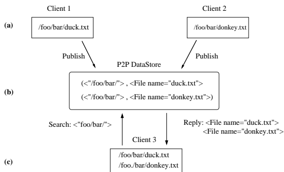
Figure 2: (a) Two users publishing different files to the same directory; (b) The meta-inodes are published to PlanetP; (c) A merged view of the directory is achieved by querying PlanetP and then contacting the appropriate peers for the meta-inodes.
