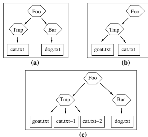
Figure 1: (a, b) Two local directory structures, and (c) the merged view in the global directory structure.
