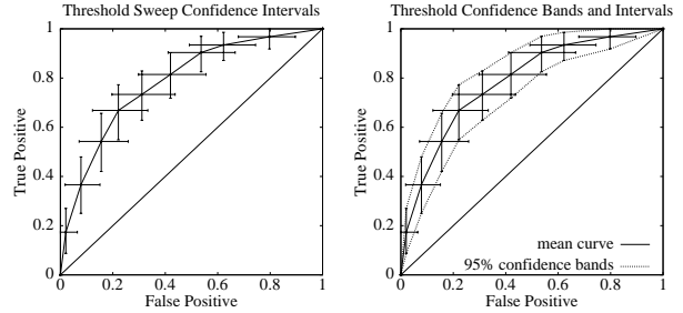
Figure 3. Transforming threshold sweep into confidence bands.
