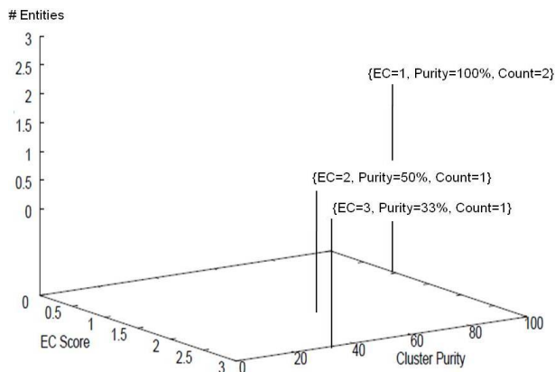
Figure 7. 3-D Entity Composition Histograms
