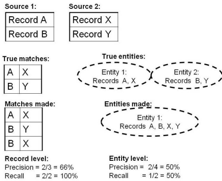
Figure 4. Misleading Record Linkage Metrics
