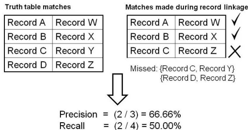
Figure 3. Record Linkage Metrics
