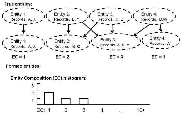
Figure 6. Entity Composition Histogram
