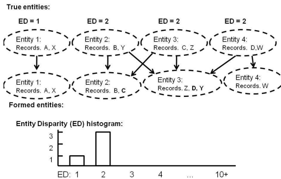
Figure 5. Entity Distribution Histogram
