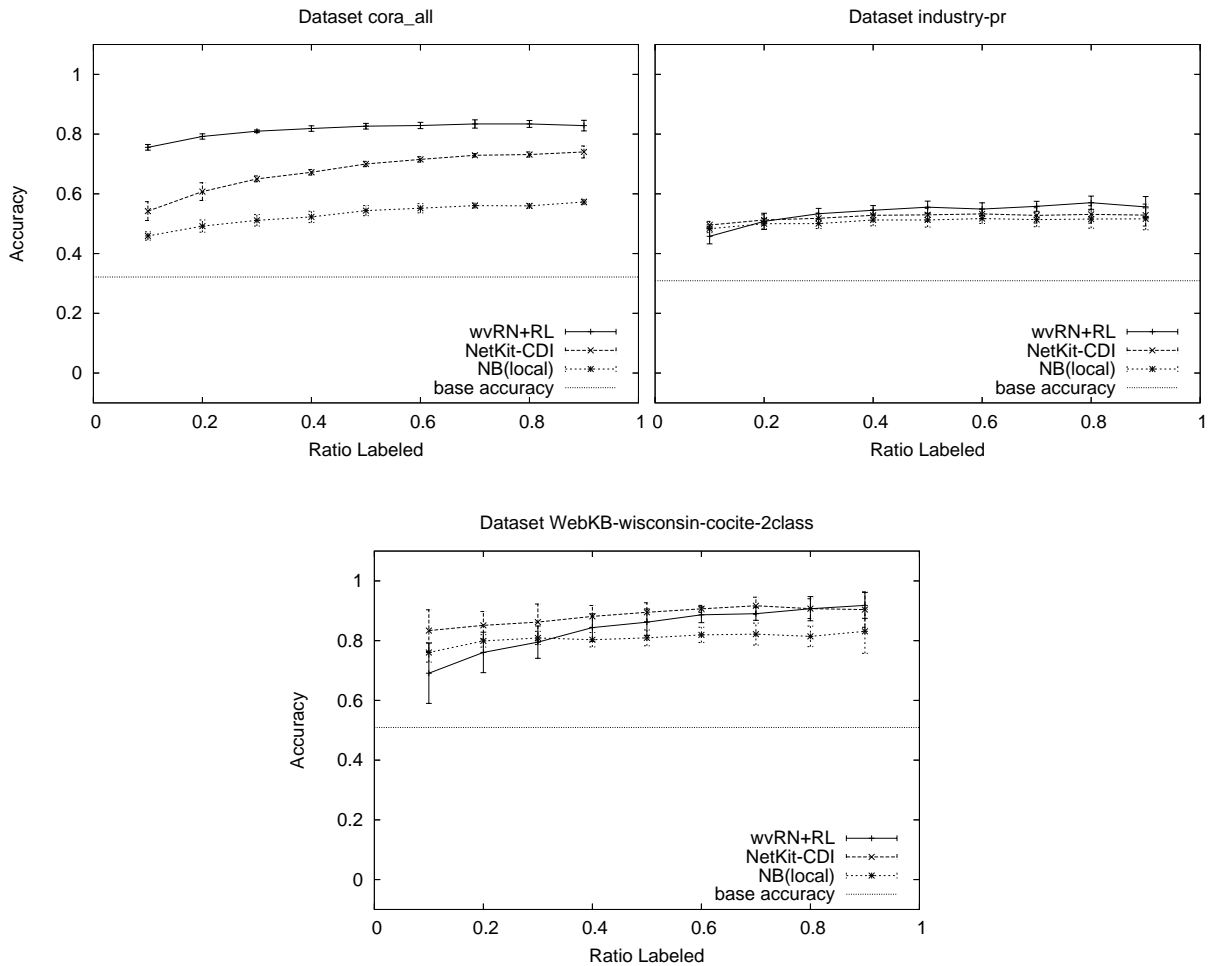
Figure 6: Comparisons of wvRN-RL (relaxation labeling), a reimplement of the method of Chakrabarti et al. (NetKit-CDI), and a local-only naive Bayes classifier (NB(local)).
